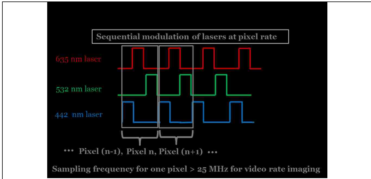
Figure 39 Pixel-sequential Imaging. Compared to Frame-sequential Imaging, which switches lasers on and off at video frame rate (e.g., 30 Hz), the pixel-sequential imaging requires modulation of lasers at pixel acquisition frequency. Standard wide-field high-resolution SFE system operates at a pixel sampling frequency of 25 MHz, therefore, for concurrent imaging of 3 fluorophores, 75 MHz modulation will be needed.
