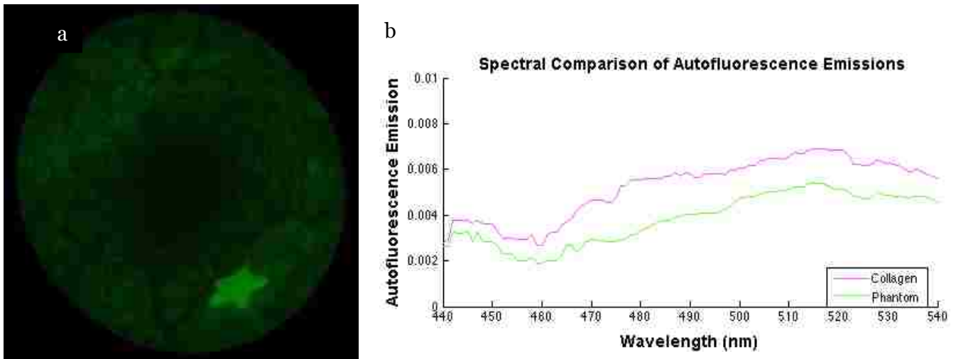
Figure 41 (a) Normalized fluorescence emissions captured by the SFE between 500-540nm after excitation at 442nm. The star shape is a FL-in-polymer dye target with a concentration of 1\mu\text{M} where as the background fluorescence is due to the embedded collagen AF. Image analysis shows the target to background signal ratio was 4:1. (b) Comparison of AF emissions shows that the phantom fluorescence emission is similar to that of pure collagen. Concerns that the excitation fiber exhibits autofluorescence was tested using a spectrometer (USB2000+, Ocean Optics, Inc). No autofluorescence signal was detected with the laser excitation power used in the current study.
